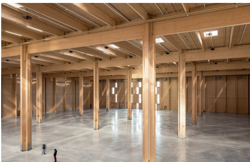
Complete timber hall of the iLogistics Centre in Fischamend
