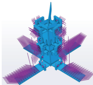
World of Volvo: central bending-resistant steel node for very high forces
