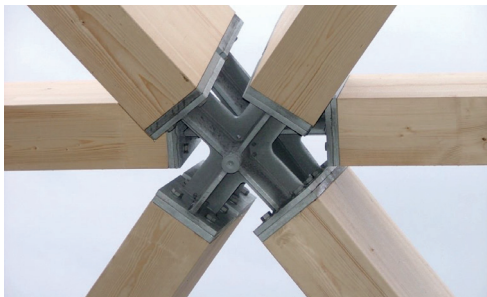
Crossrail station, rigid connection hub Quickest assembly in cantilever construction (unsupported)
