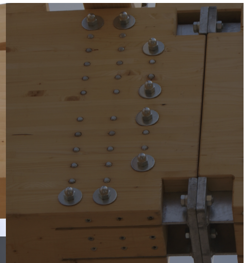
GVZ Ingolstadt rail track roofing, trussed arched beams, completely pre-assembled at factory
