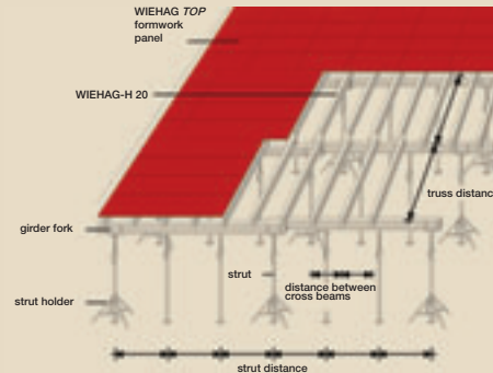
Example of ceiling formwork
